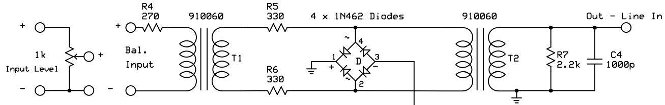
Compressor Limiter P/N 550109
